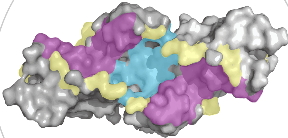
ARCUS protein with DNA interface in color
